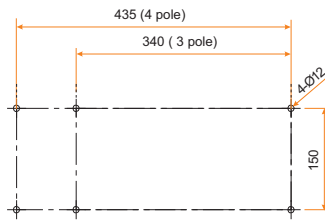
Assembling Gauge
