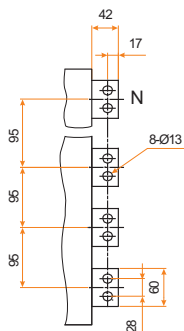
Busbar Connections
