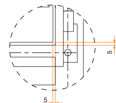
Panel Frame
