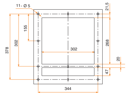
Panel Frame
