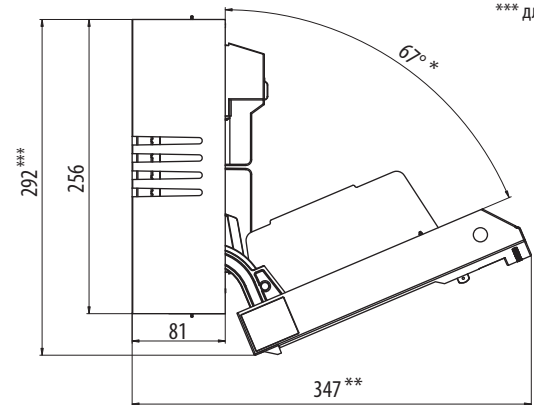
FH2-1S/F и FH2-3S/F
