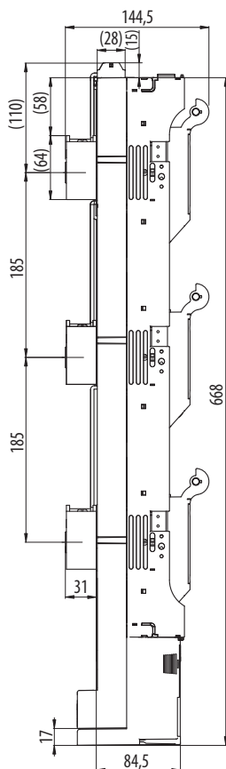
FSD00-31D-FC-M...
