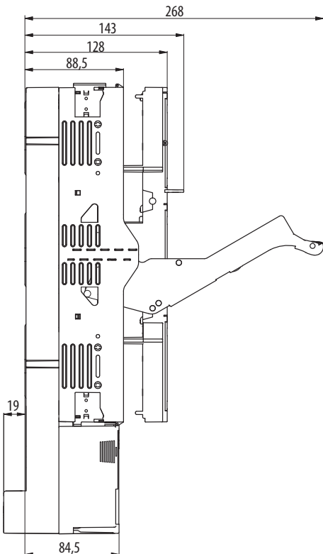
FSD00-33K-FC
