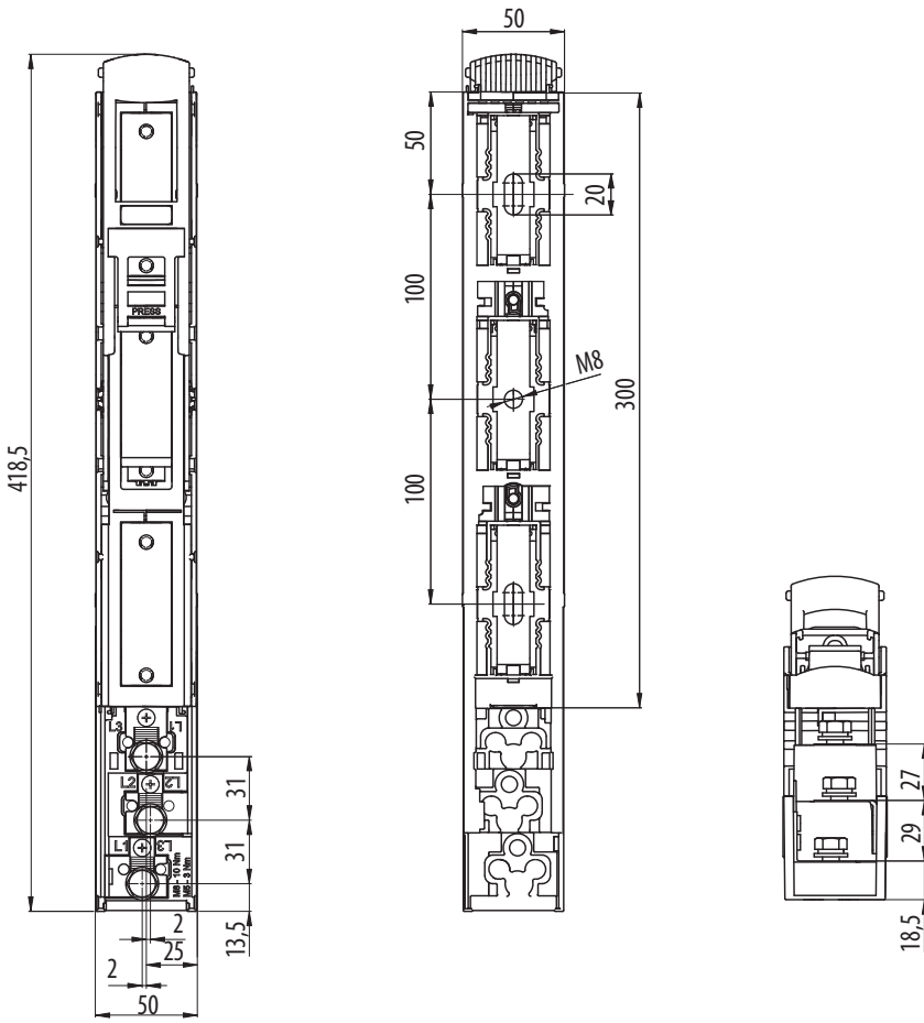
FSD00-33K-F
